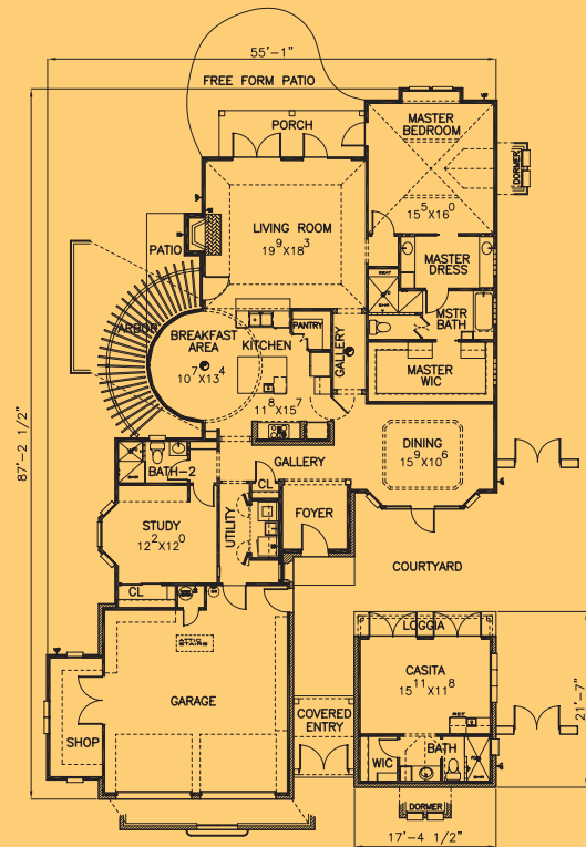
MAIN HOUSE FLOOR PLAN 2111 SQ. FT.
